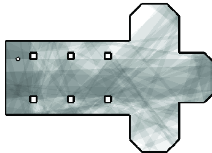
Fig. 2: Superposition of beams in a complex 2D environment (only reflections up to the 2 nd order are visualized).
